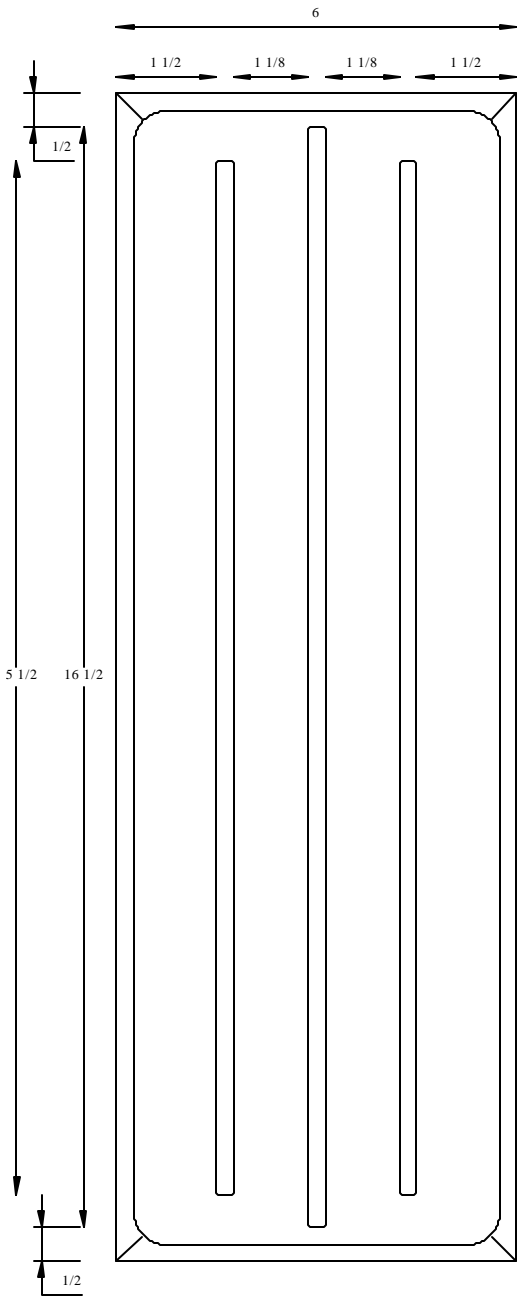
Door 3/4" thick
